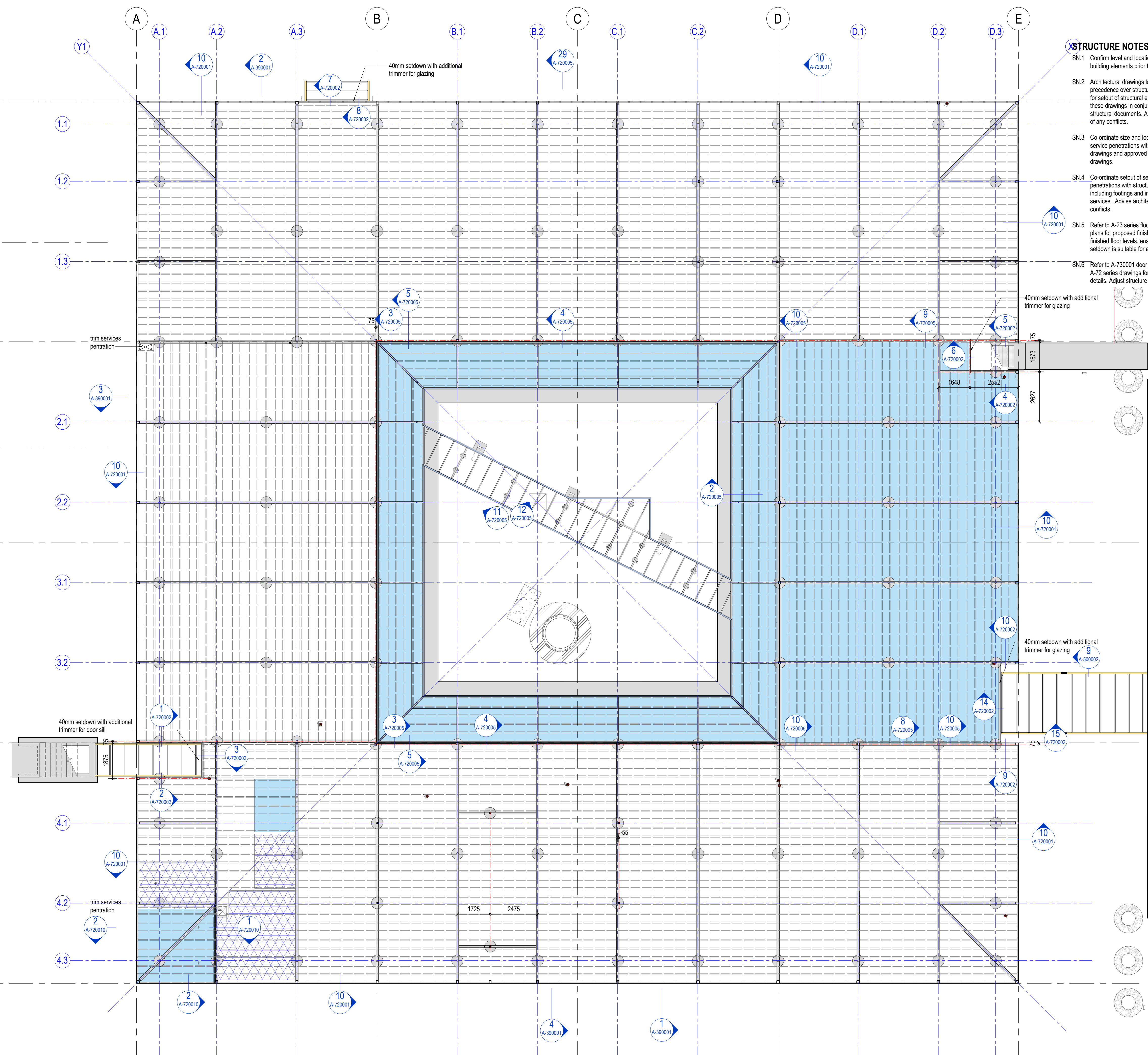
1 Sub-Floor Plan 1:100
